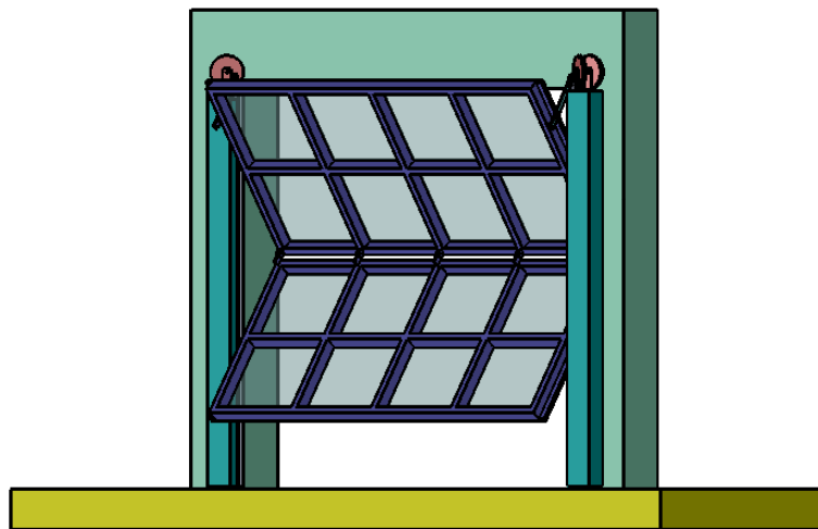
INSIDE VIEW - DOOR IN OPERATION
