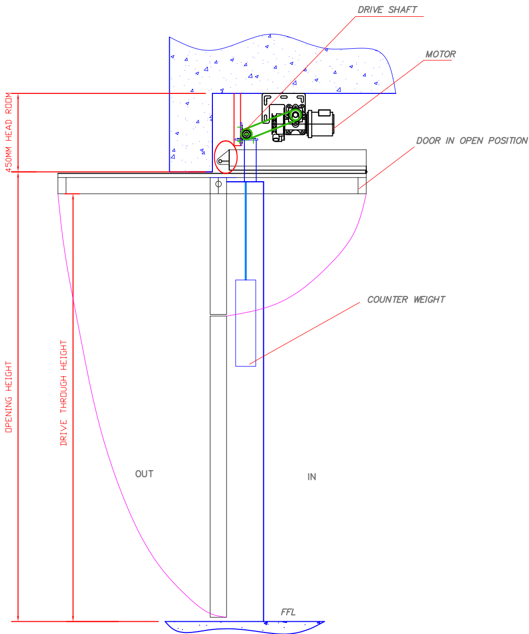
SIDE VIEW
