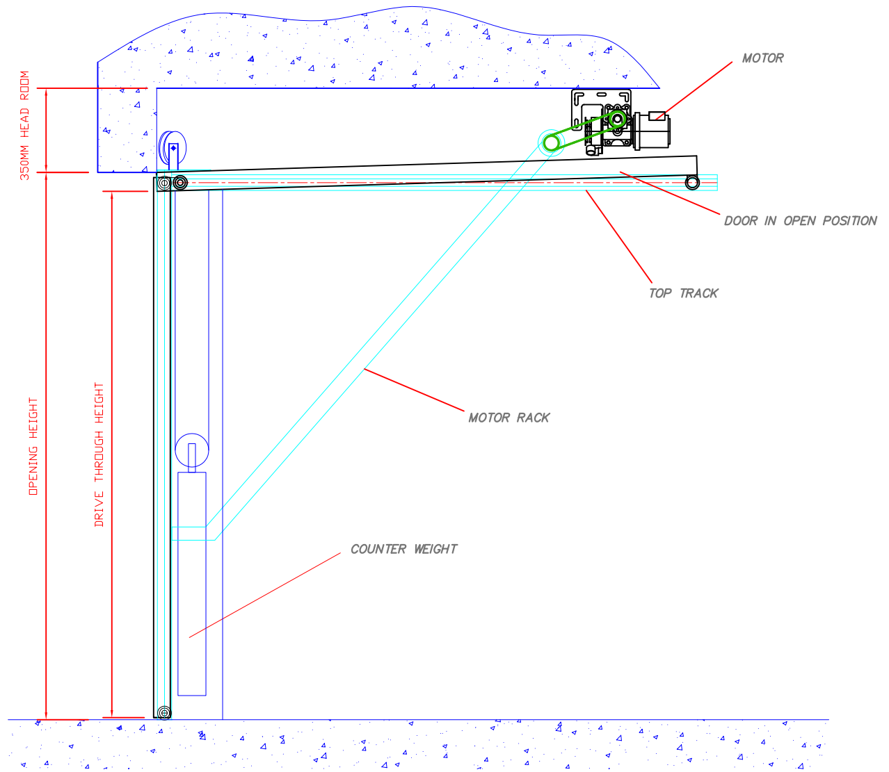
SIDE VIEW
