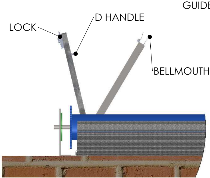
DETAIL B
